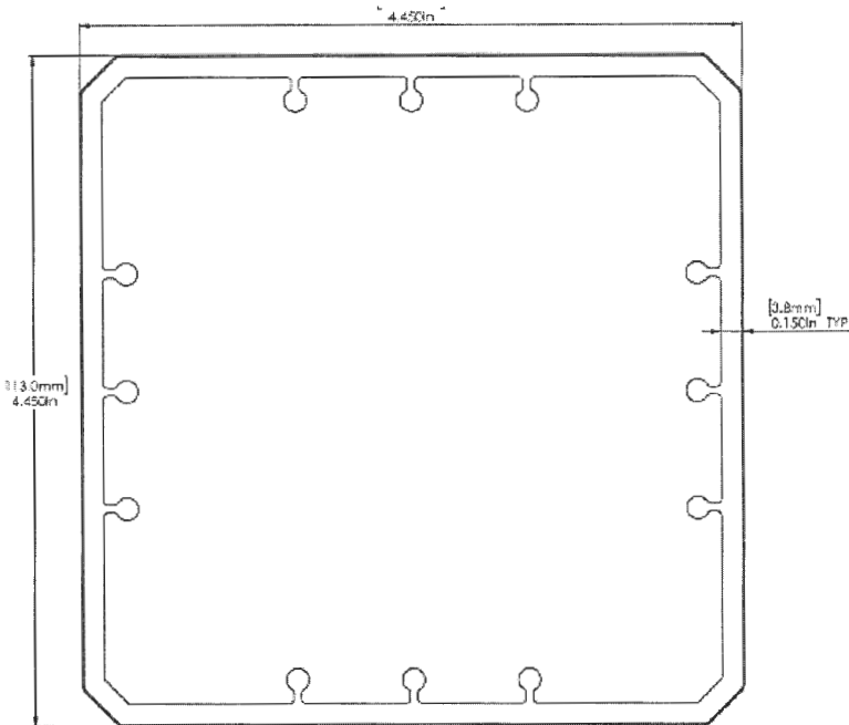
FIGURE 6 – 4X4 POST SLEEVE
