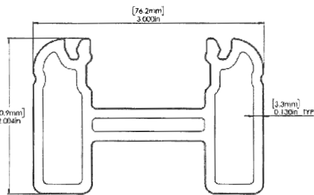
Bottom (Universal) Rail
