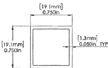
Square Aluminum Baluster
