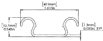
Rail Insert (For Aluminum Balusters Only)
