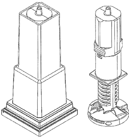
FIGURE 5 – FOOT BLOCK
