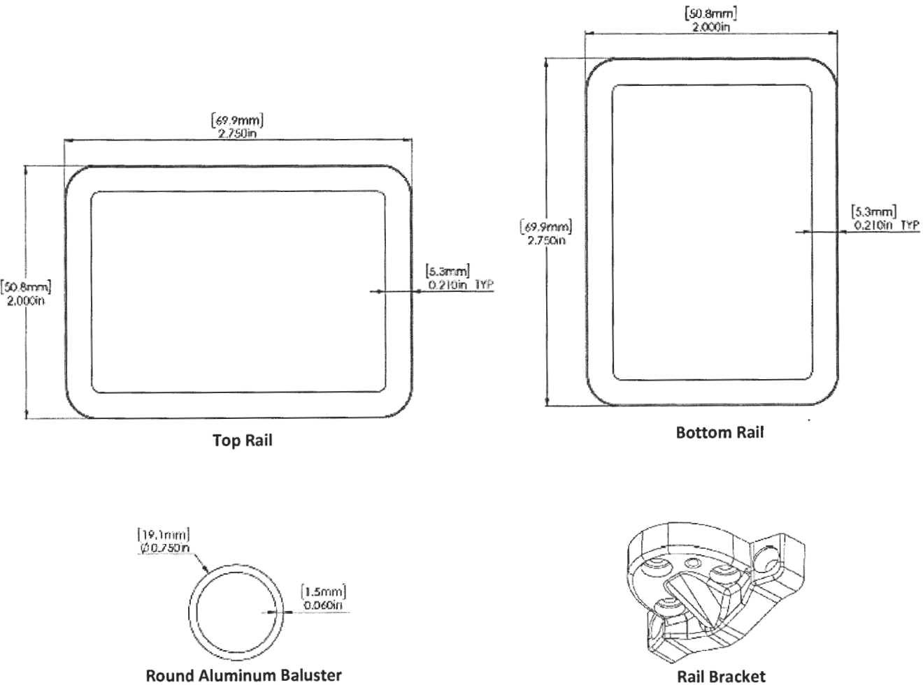
FIGURE 4 – TREX® SELECT®/ENHANCE® GUARDRAIL COMPONENTS
