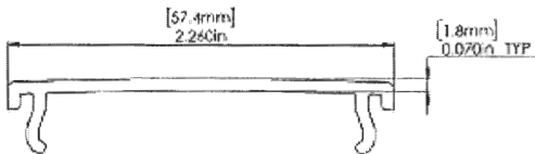
Baluster Spacer
