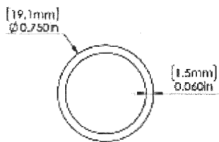
Round Aluminum Baluster
